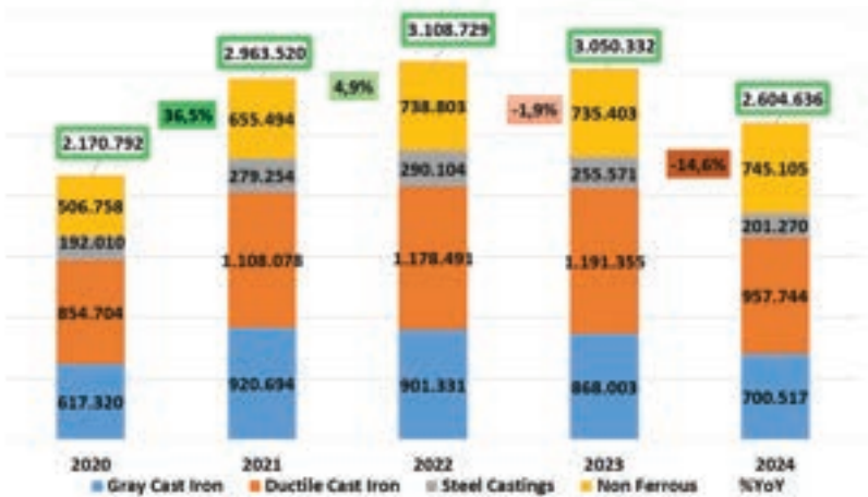
Turkey Metal Casting Production Annual Production Breakdown (tons/year) *Source: TÜDÖKSAD
